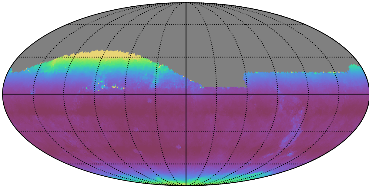
ddf_loaded_fl1_v3.4_10yrs Yr 1 all bands: Median airmass
