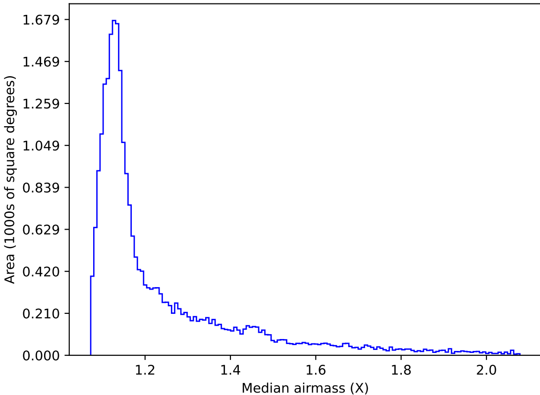
ddf_loaded_fl1_v3.4_10yrs Yr 1 all bands: Median airmass
