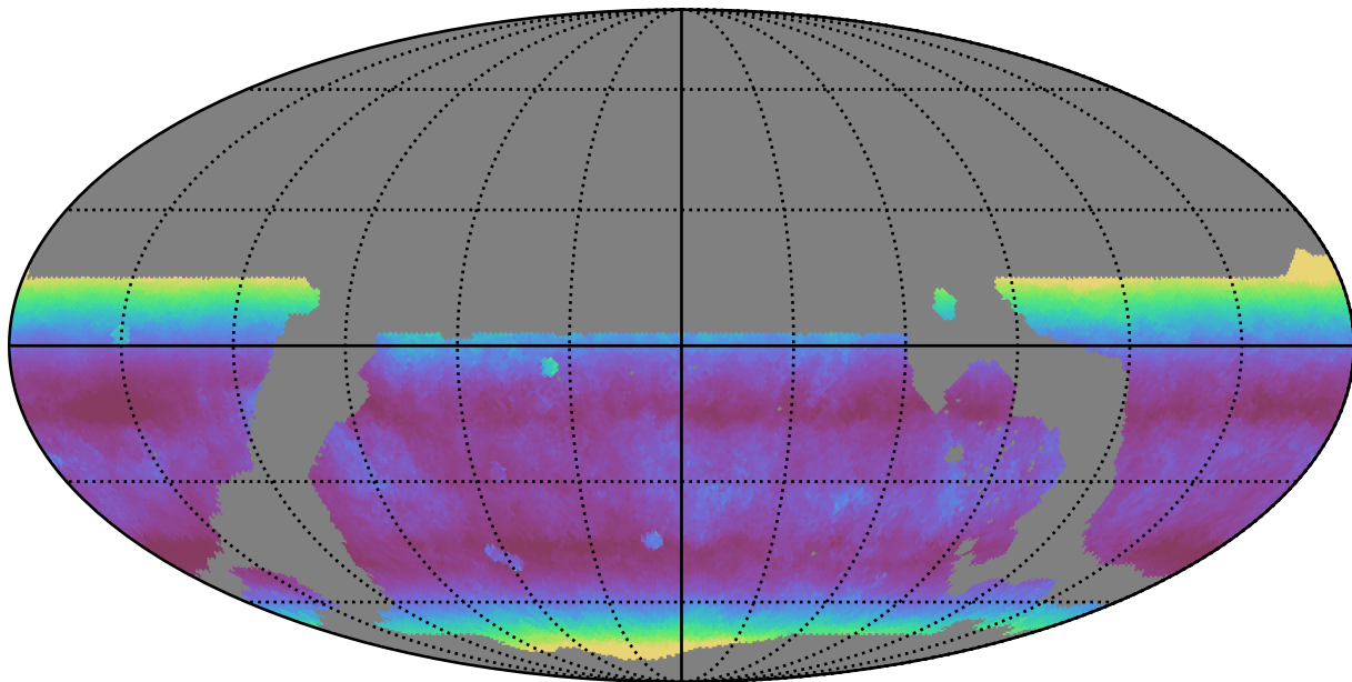
ddf_loaded_fl1_v3.4_10yrs WFD z band: Median airmass
