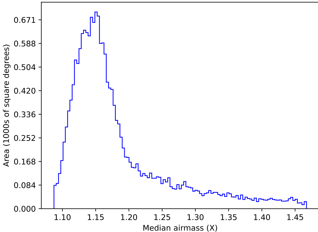
ddf_loaded_fl1_v3.4_10yrs WFD z band: Median airmass
