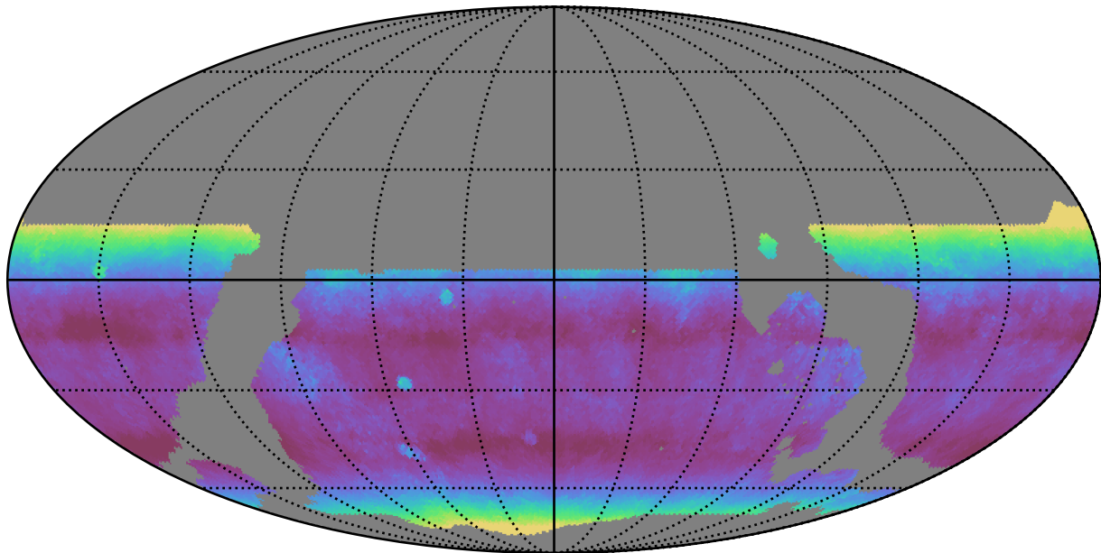
ddf_loaded_fl1_v3.4_10yrs WFD y band: Median airmass
