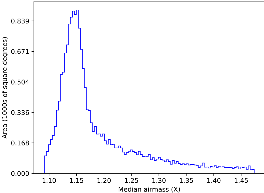
ddf_loaded_fl1_v3.4_10yrs WFD y band: Median airmass
