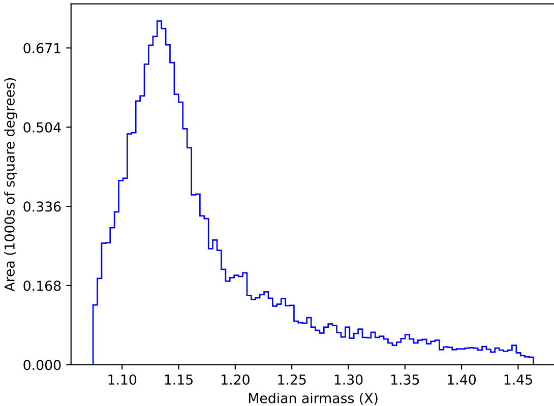
ddf_loaded_fl1_v3.4_10yrs WFD u band: Median airmass
