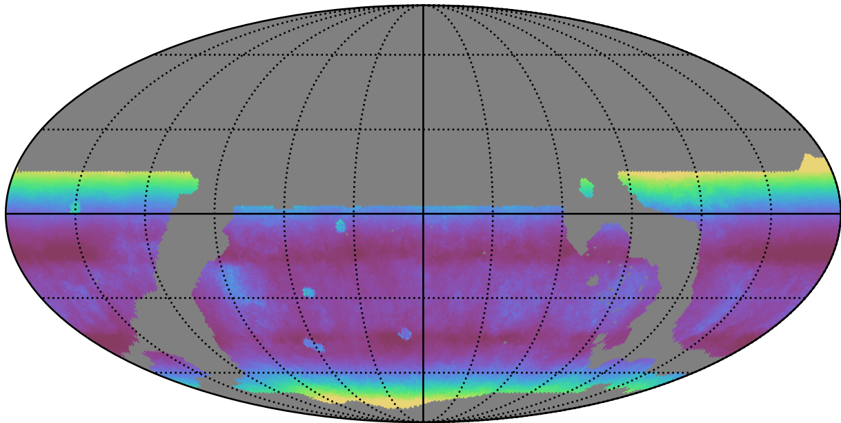
ddf_loaded_fl1_v3.4_10yrs WFD r band: Median airmass
