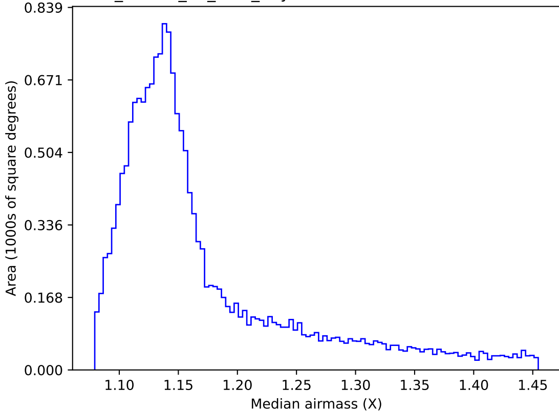
ddf_loaded_fl1_v3.4_10yrs WFD i band: Median airmass
