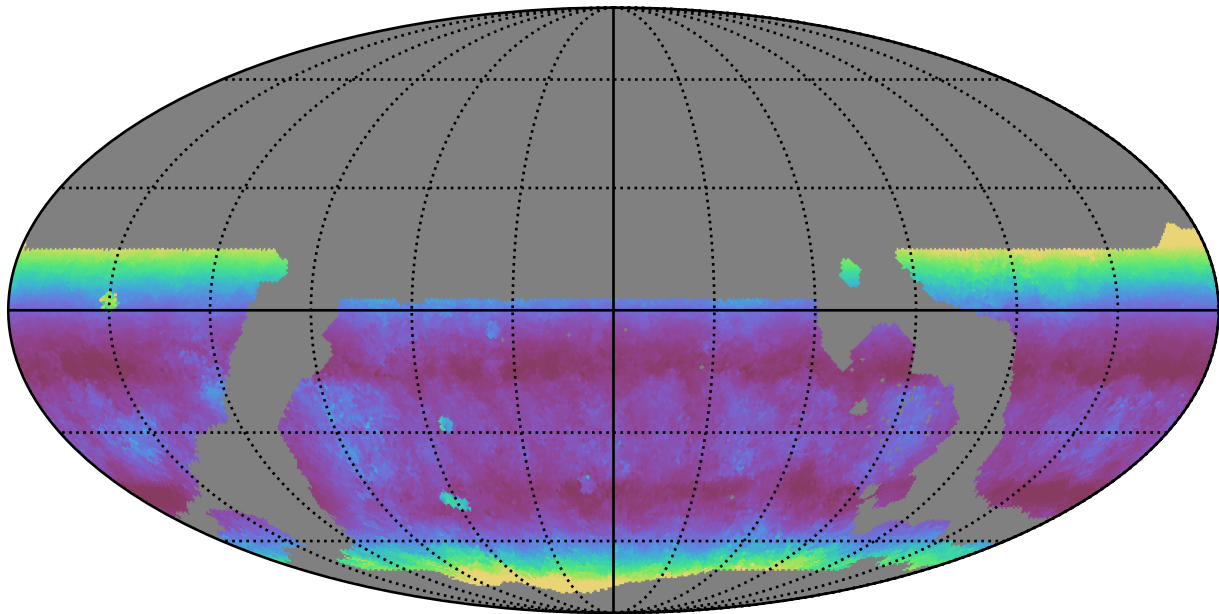
ddf_loaded_fl1_v3.4_10yrs WFD g band: Median airmass
