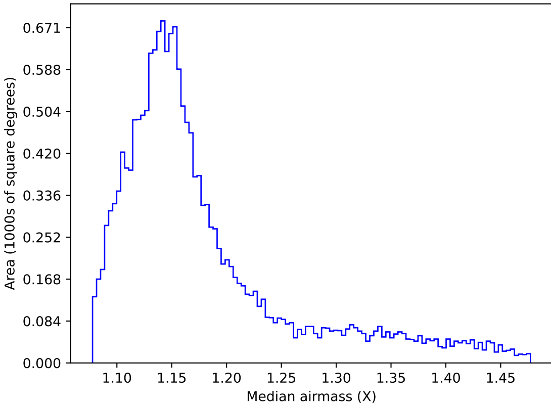
ddf_loaded_fl1_v3.4_10yrs WFD g band: Median airmass
