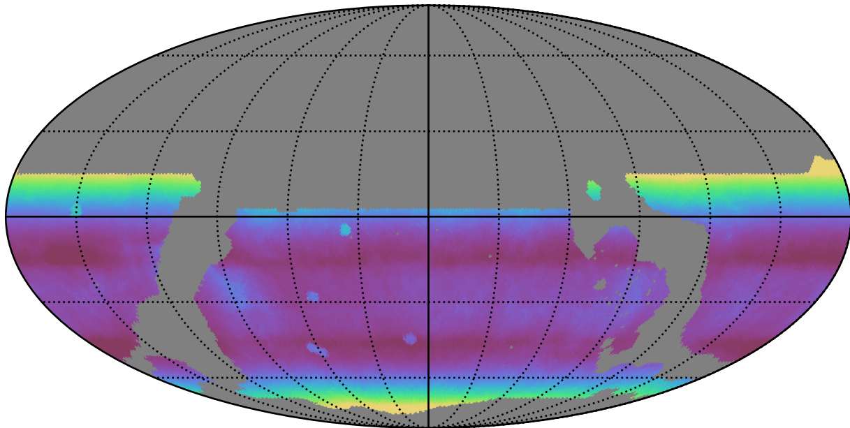
ddf_loaded_fl1_v3.4_10yrs WFD all bands: Median airmass
