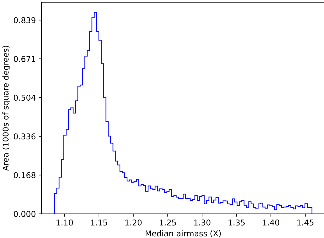
ddf_loaded_fl1_v3.4_10yrs WFD all bands: Median airmass
