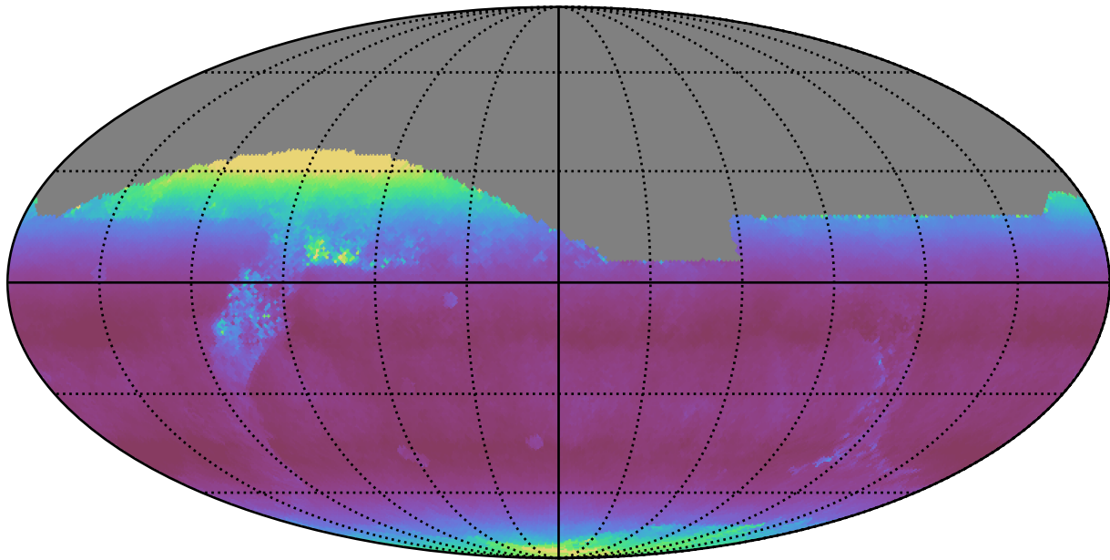
ddf_loaded_fl1_v3.4_10yrs All sky z band: Median airmass
