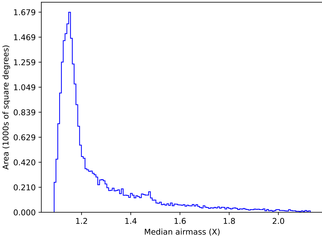
ddf_loaded_fl1_v3.4_10yrs All sky z band: Median airmass
