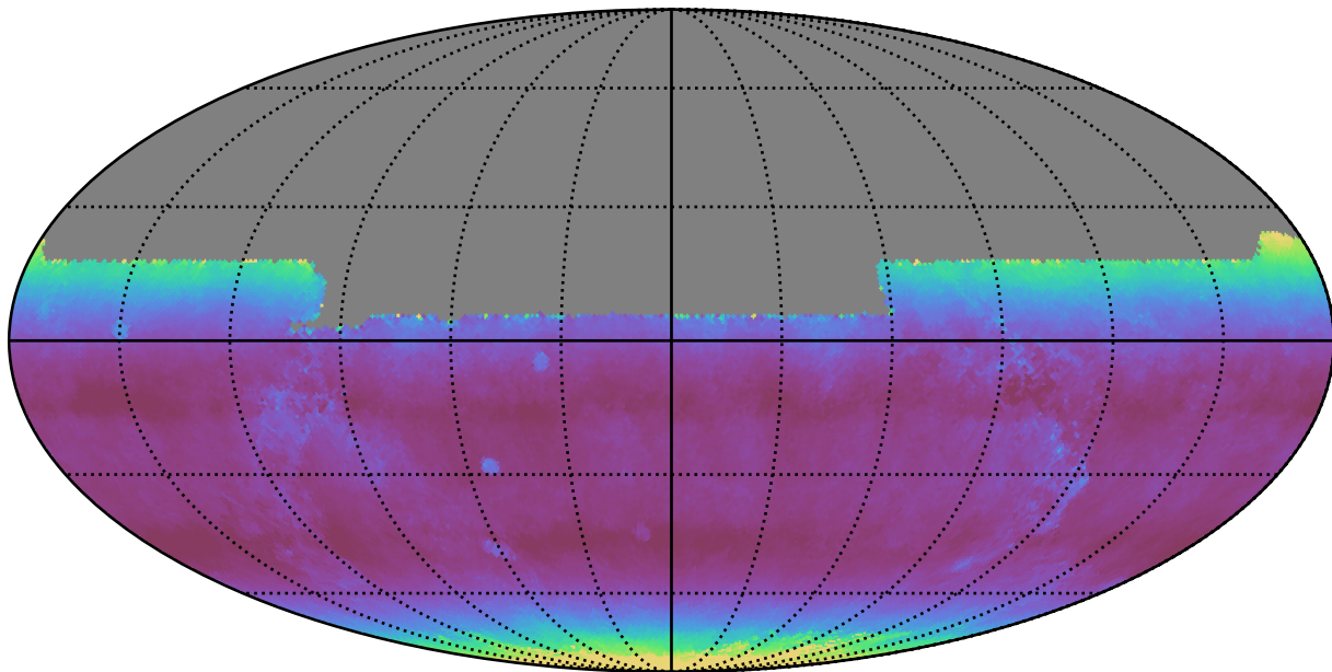
ddf_loaded_fl1_v3.4_10yrs All sky y band: Median airmass
