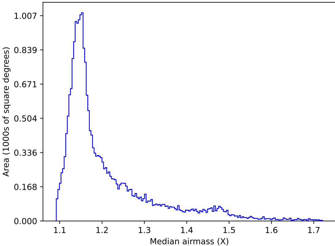
ddf_loaded_fl1_v3.4_10yrs All sky y band: Median airmass
