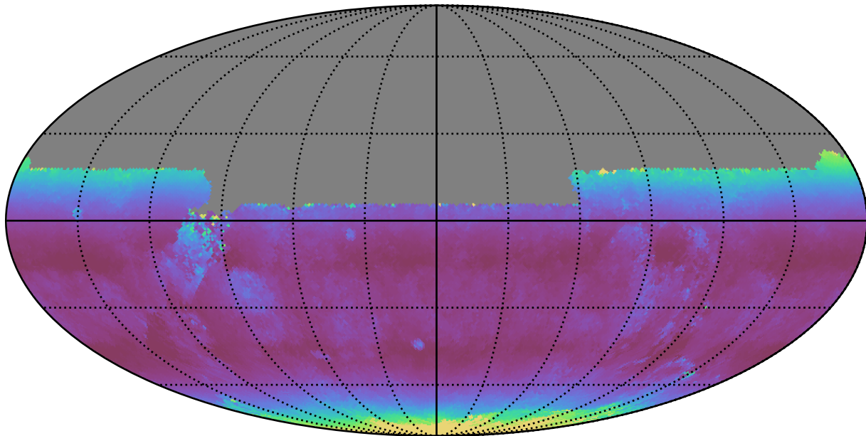
ddf_loaded_fl1_v3.4_10yrs All sky u band: Median airmass
