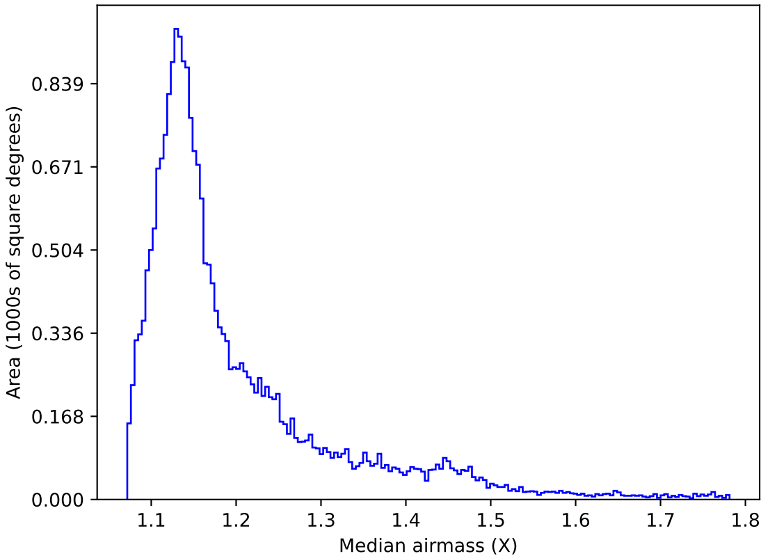
ddf_loaded_fl1_v3.4_10yrs All sky u band: Median airmass
