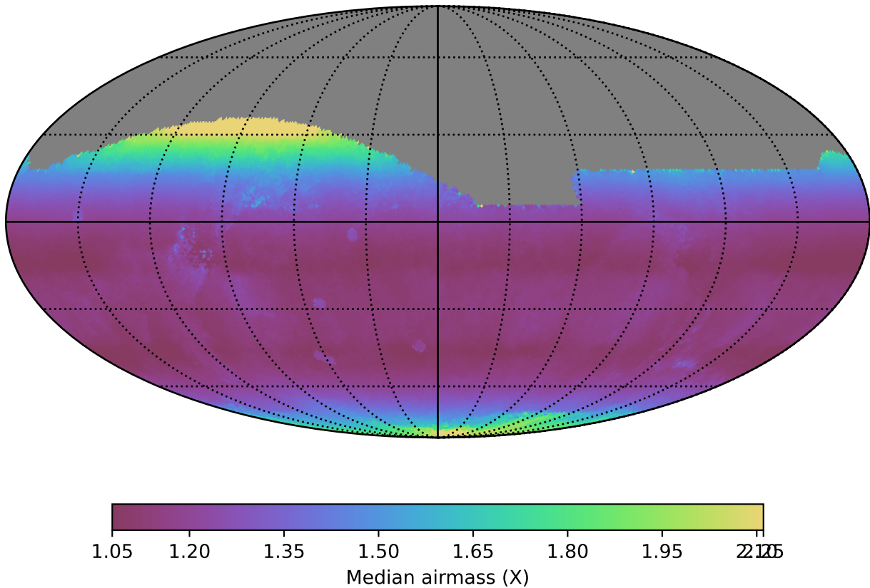
ddf_loaded_fl1_v3.4_10yrs All sky r band: Median airmass
