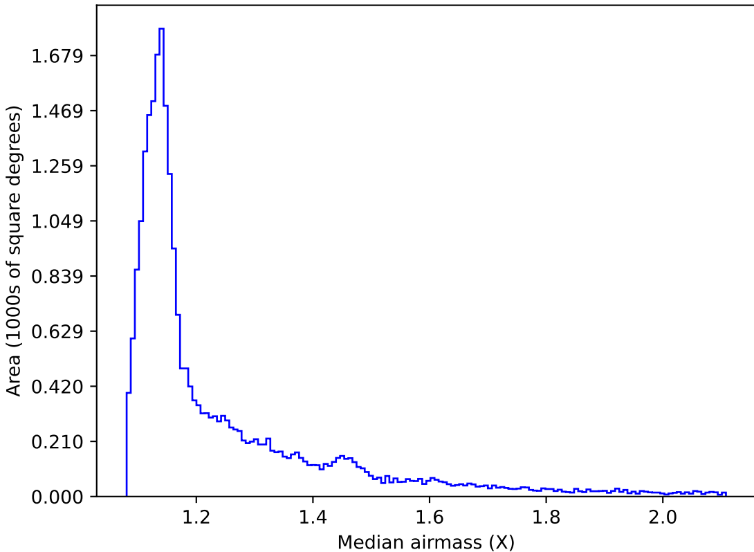
ddf_loaded_fl1_v3.4_10yrs All sky i band: Median airmass
