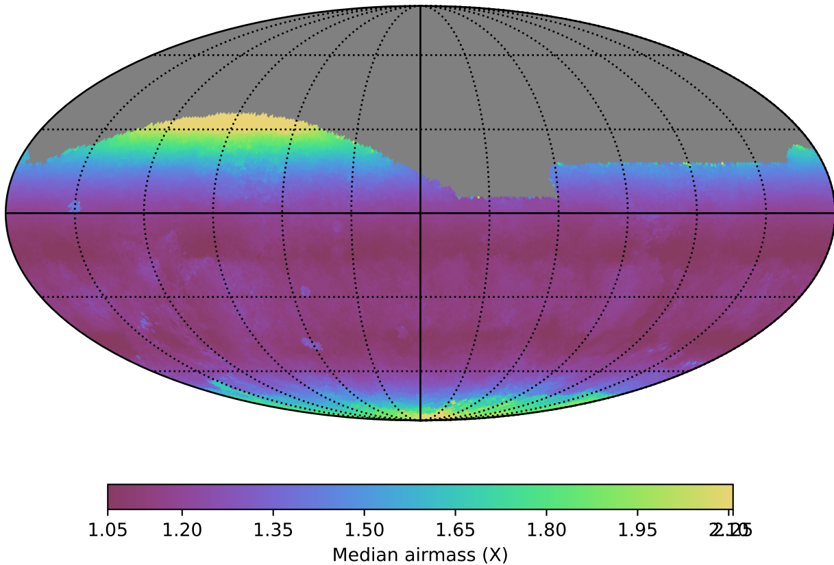
ddf_loaded_fl1_v3.4_10yrs All sky g band: Median airmass
