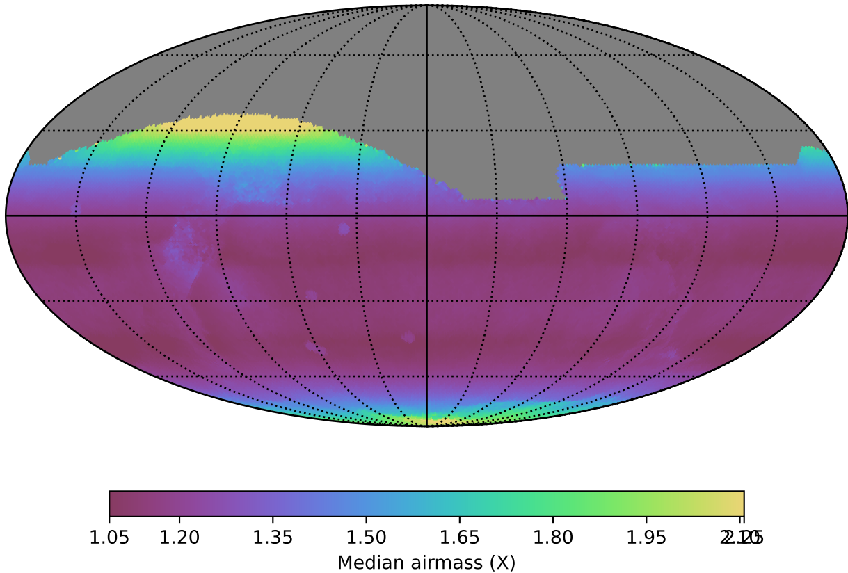
ddf_loaded_fl1_v3.4_10yrs All sky all bands: Median airmass
