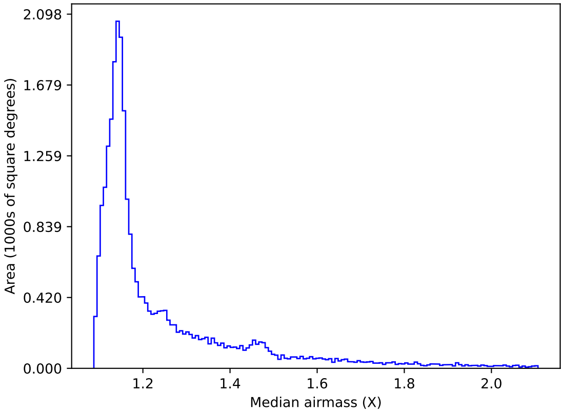
ddf_loaded_fl1_v3.4_10yrs All sky all bands: Median airmass
