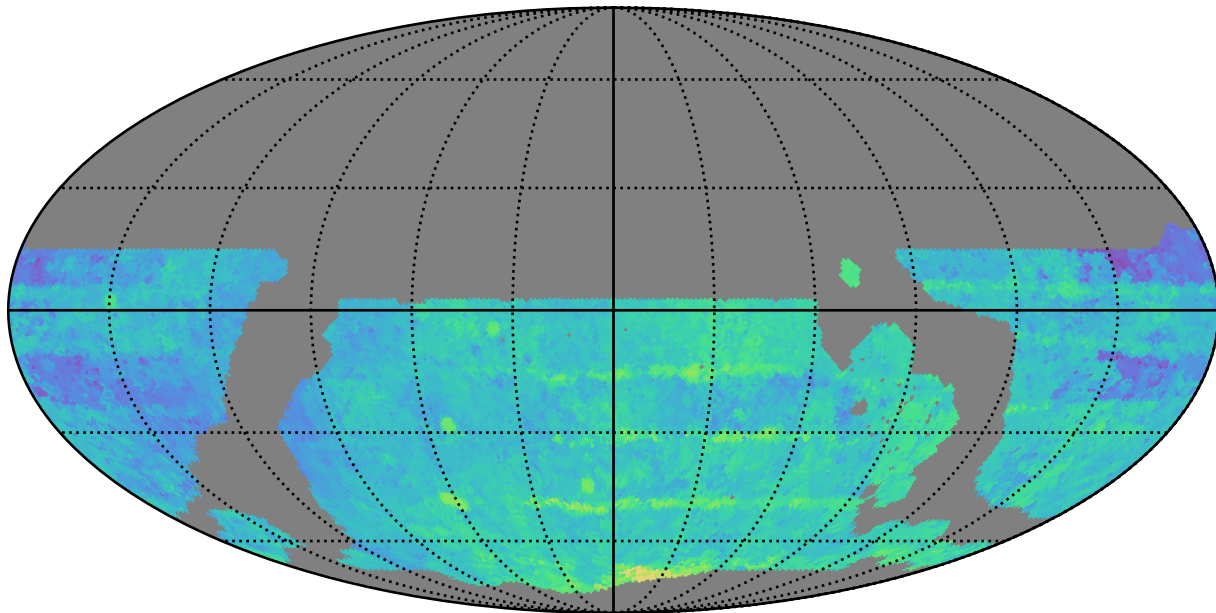
ddf_loaded_fl1_v3.4_10yrs WFD z band: Median Season Length
