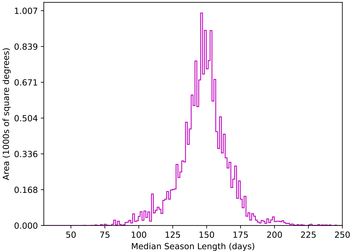
ddf_loaded_fl1_v3.4_10yrs WFD z band: Median Season Length
