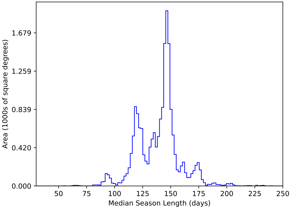
ddf_loaded_fl1_v3.4_10yrs WFD y band: Median Season Length
