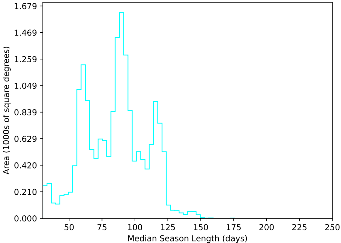
ddf_loaded_fl1_v3.4_10yrs WFD u band: Median Season Length
