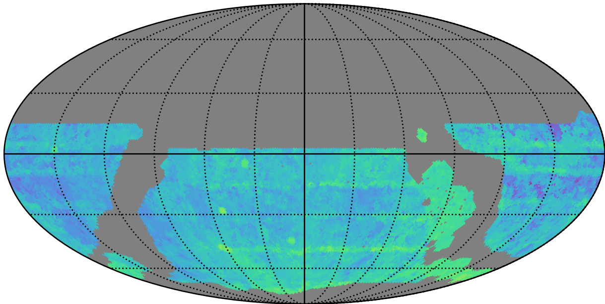
ddf_loaded_fl1_v3.4_10yrs WFD r band: Median Season Length
