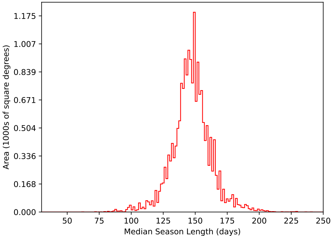
ddf_loaded_fl1_v3.4_10yrs WFD i band: Median Season Length
