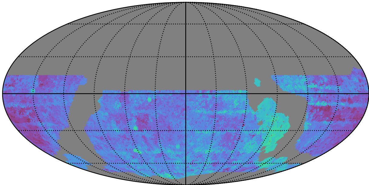
ddf_loaded_fl1_v3.4_10yrs WFD g band: Median Season Length
