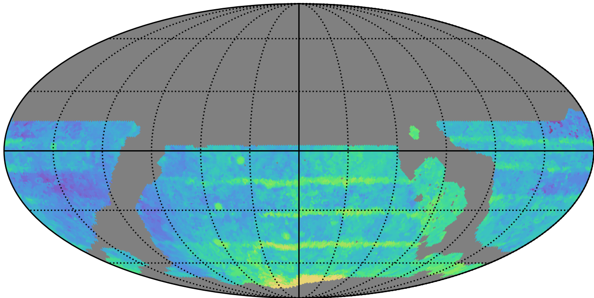
ddf_loaded_fl1_v3.4_10yrs WFD all bands: Median Season Length
