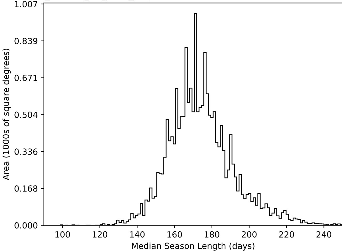
ddf_loaded_fl1_v3.4_10yrs WFD all bands: Median Season Length
