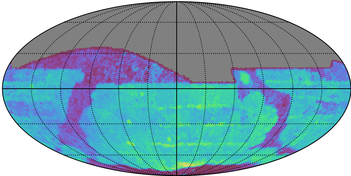
ddf_loaded_fl1_v3.4_10yrs All sky z band: Median Season Length
