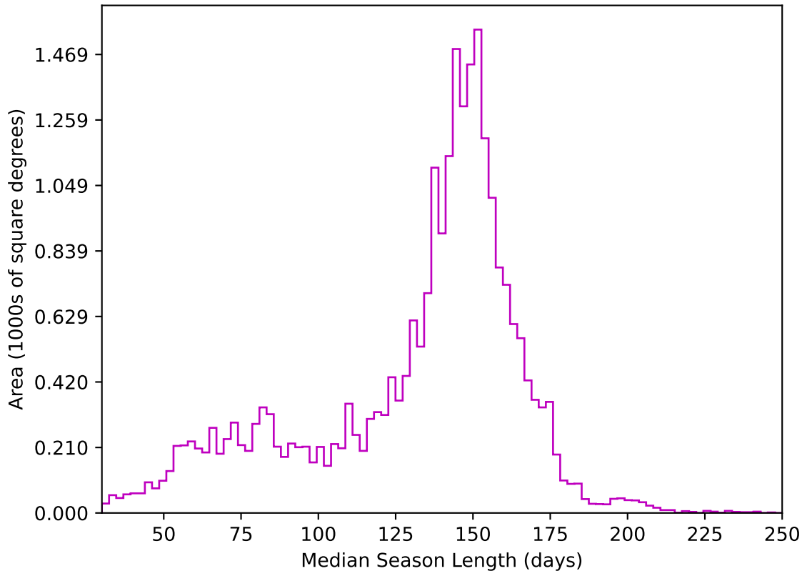
ddf_loaded_fl1_v3.4_10yrs All sky z band: Median Season Length
