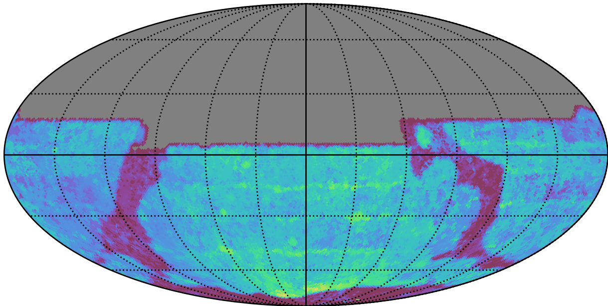
ddf_loaded_fl1_v3.4_10yrs All sky y band: Median Season Length
