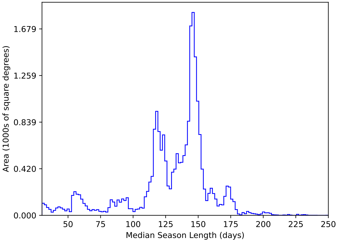
ddf_loaded_fl1_v3.4_10yrs All sky y band: Median Season Length
