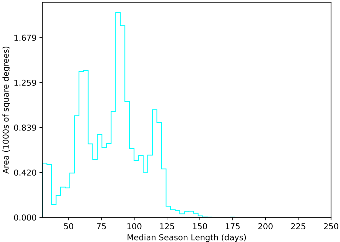
ddf_loaded_fl1_v3.4_10yrs All sky u band: Median Season Length
