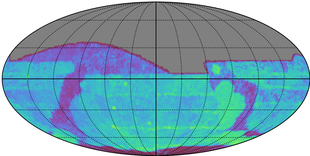
ddf_loaded_fl1_v3.4_10yrs All sky r band: Median Season Length
