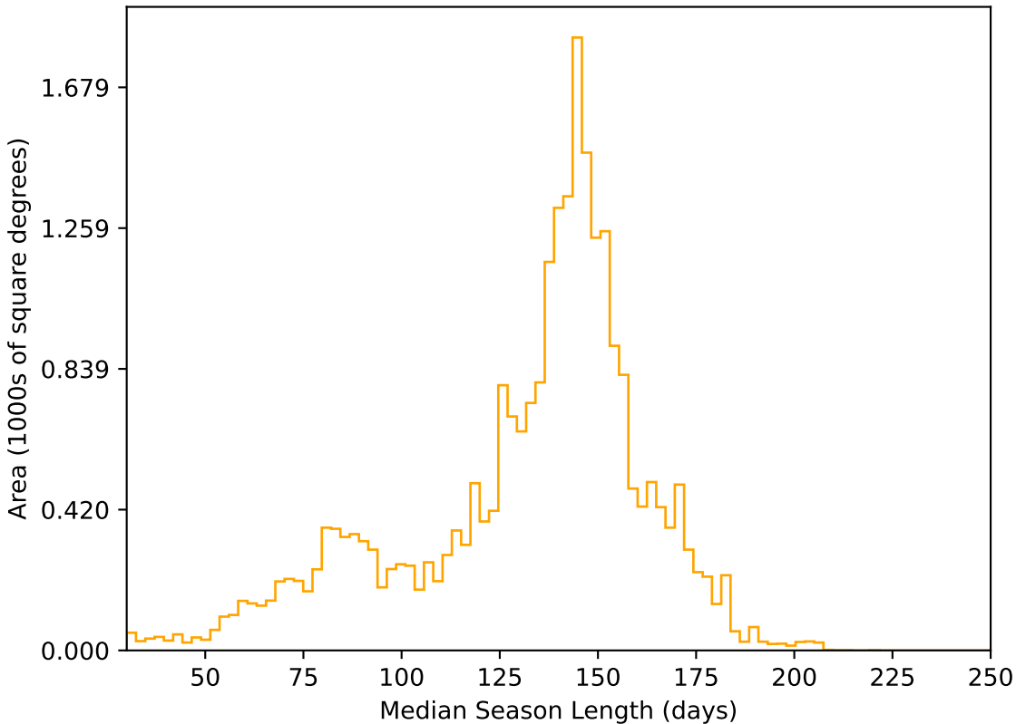
ddf_loaded_fl1_v3.4_10yrs All sky r band: Median Season Length
