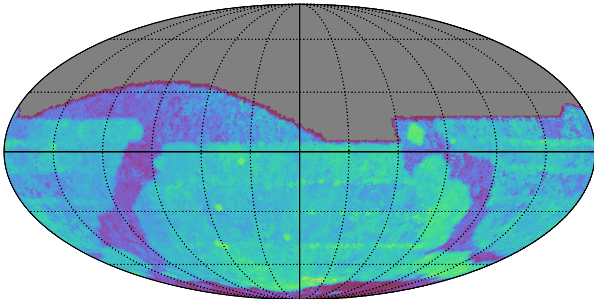
ddf_loaded_fl1_v3.4_10yrs All sky i band: Median Season Length
