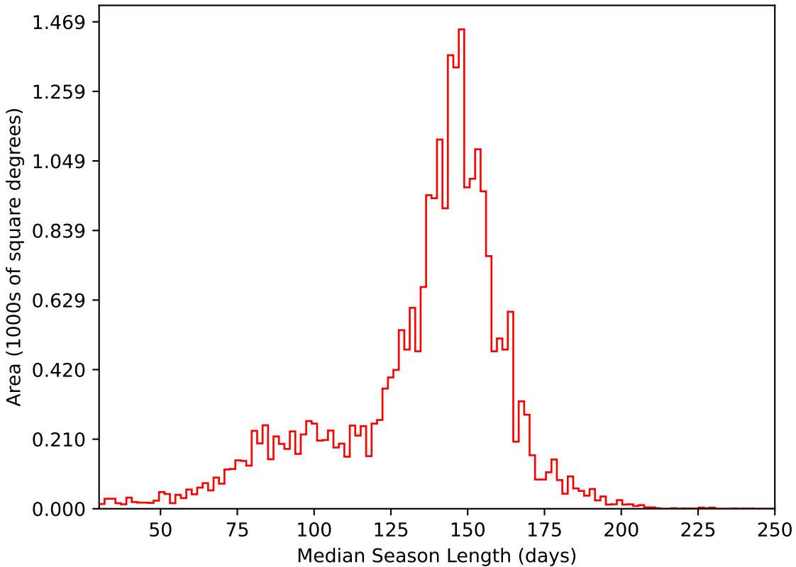
ddf_loaded_fl1_v3.4_10yrs All sky i band: Median Season Length
