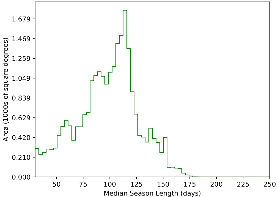
ddf_loaded_fl1_v3.4_10yrs All sky g band: Median Season Length
