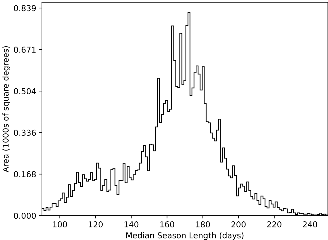
ddf_loaded_fl1_v3.4_10yrs All sky all bands: Median Season Length
