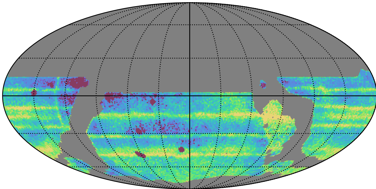
ddf_loaded_fl1_v3.4_10yrs WFD: Median Intra-Night Gap
