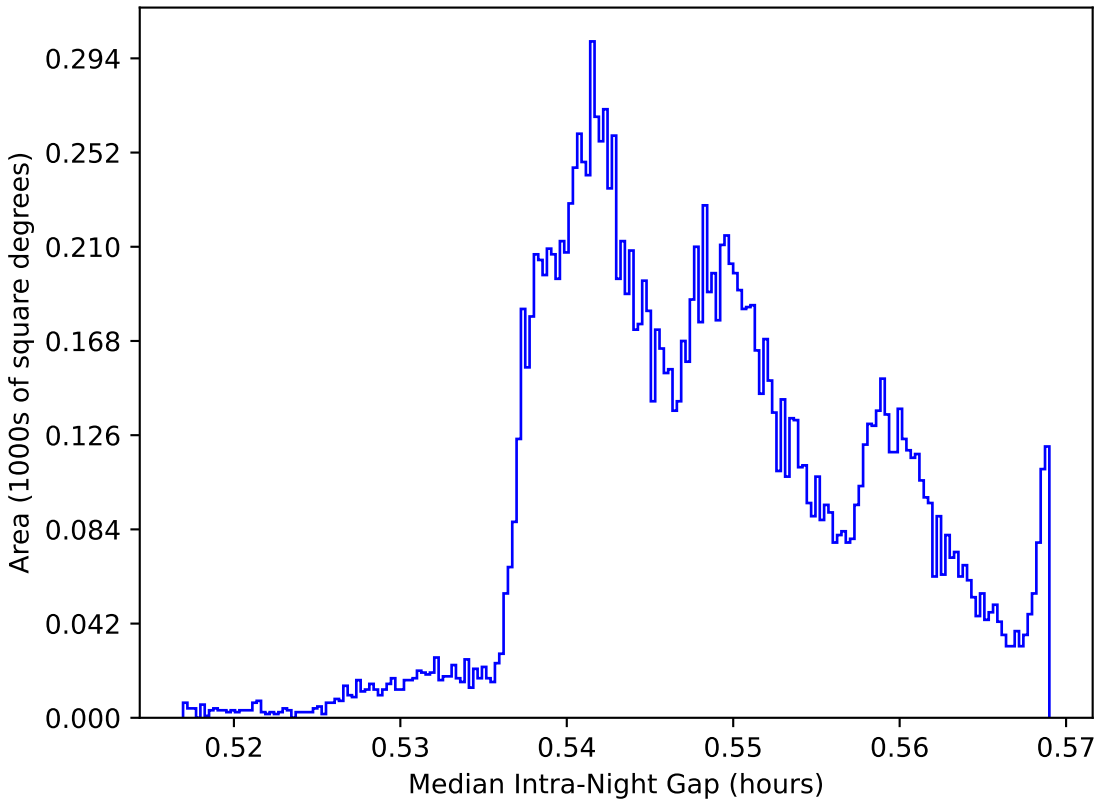
ddf_loaded_fl1_v3.4_10yrs WFD: Median Intra-Night Gap
