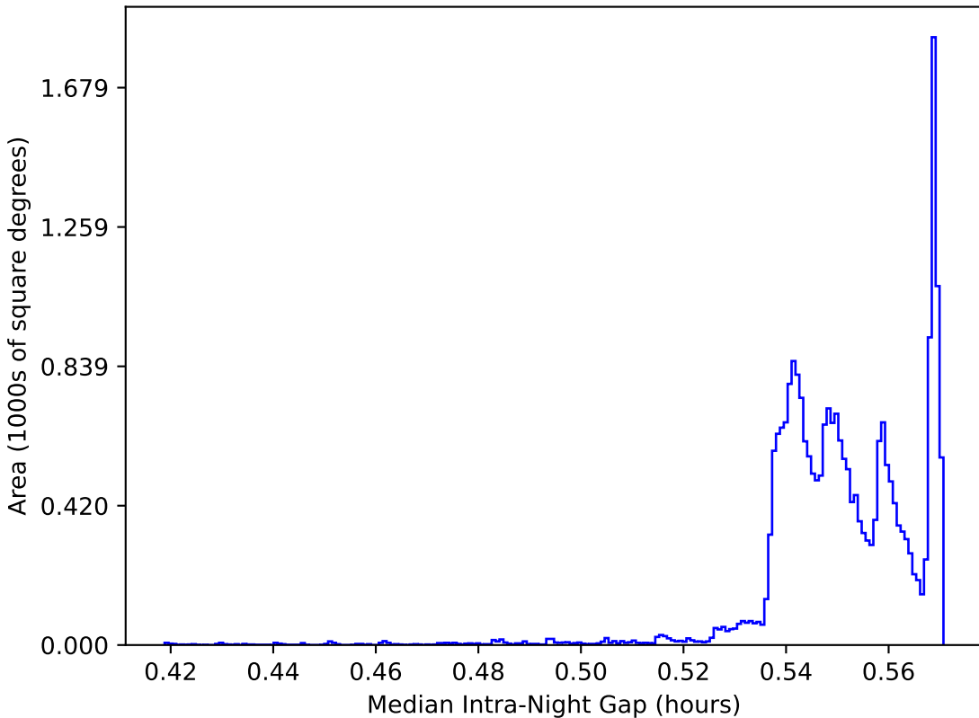
ddf_loaded_fl1_v3.4_10yrs All sky: Median Intra-Night Gap
