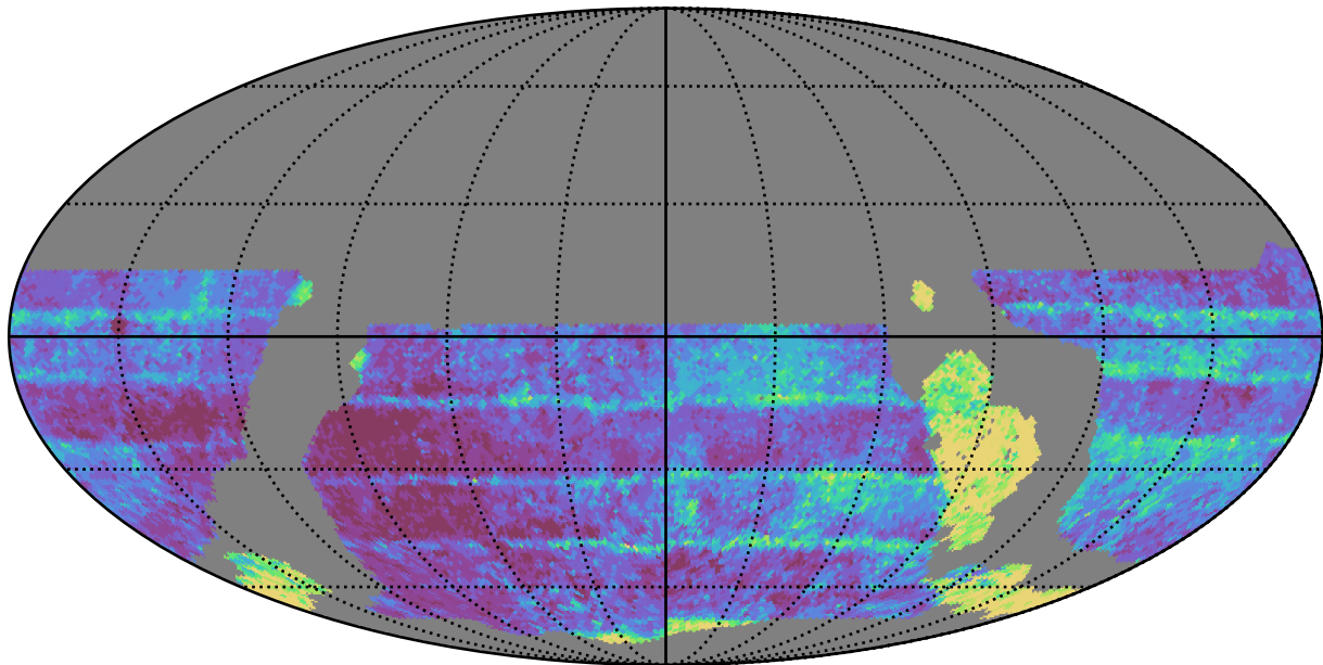
ddf_loaded_fl1_v3.4_10yrs WFD z band: Median Inter-Night Gap
