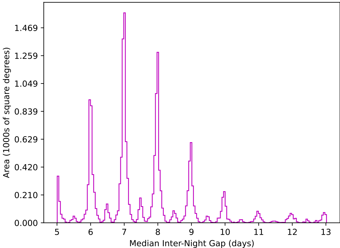
ddf_loaded_fl1_v3.4_10yrs WFD z band: Median Inter-Night Gap
