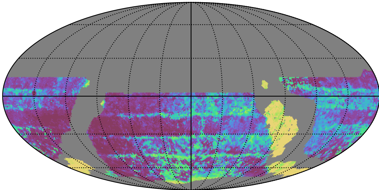
ddf_loaded_fl1_v3.4_10yrs WFD y band: Median Inter-Night Gap
